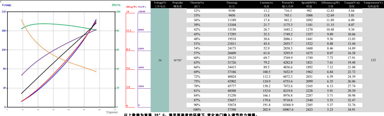
以上数据为室温 25° C、海平面高度的环境下,变化油门输入调节拉力测得。 The above data are measured under the environment of room temperature (25° C) and sea level altitude, changing the throttle input to adjust the thrust force.
