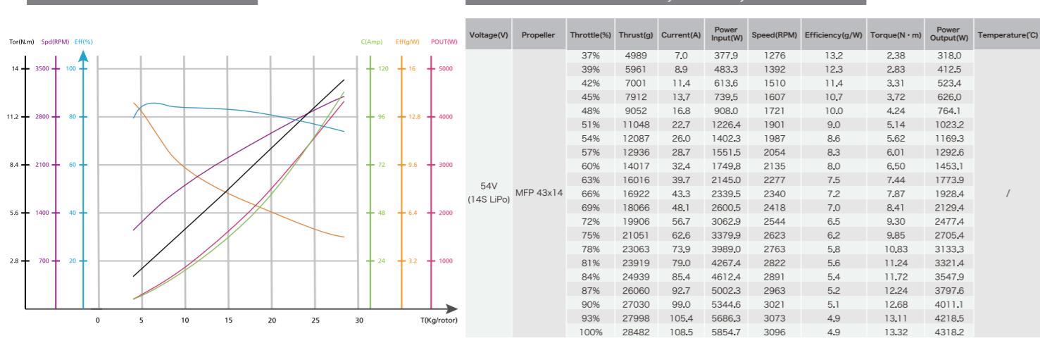
X9 Plus G2L-14S Thrust Load Curve
