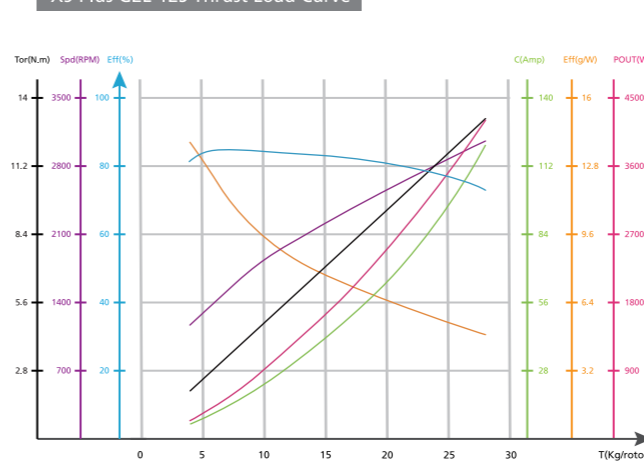
X9 Plus G2L-12S Thrust Load Curve
