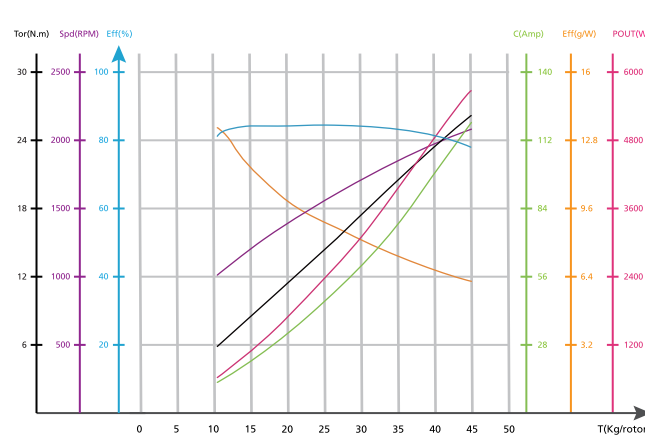
61V+MFC 57x20 Thrust Load Curve
