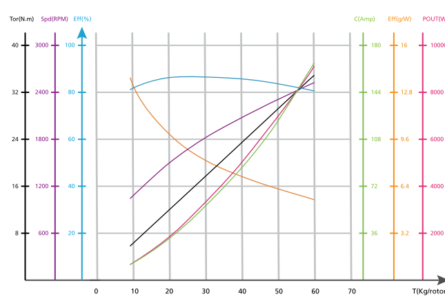
61V+MFP 56x20 Thrust Load Curve
