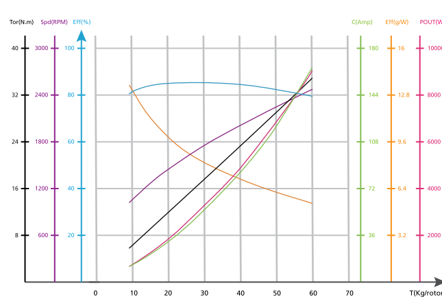
69V+MFC 57x20 Thrust Load Curve
