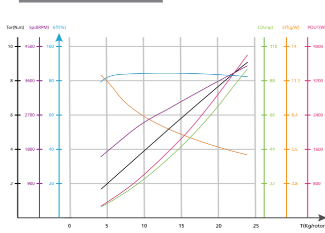
X9 G2L-12S Thrust Load Curve
