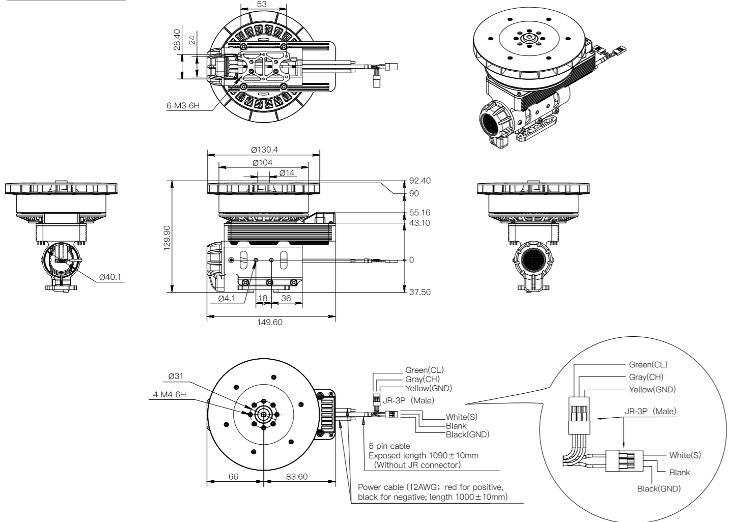
D40 Dimension Diagram
