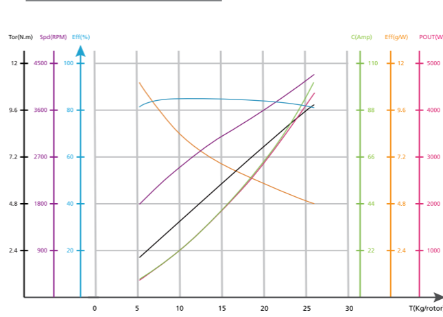
X9 G2L-14S Thrust Load Curve
