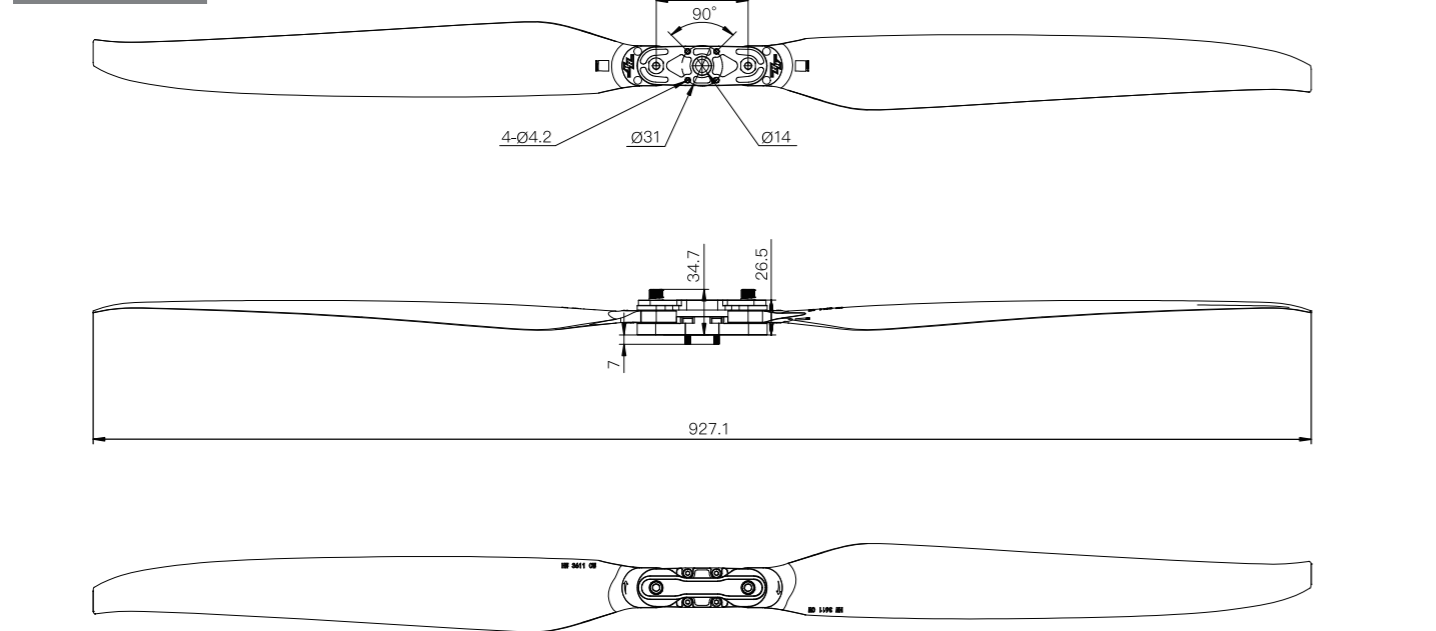
Propeller Drawings
