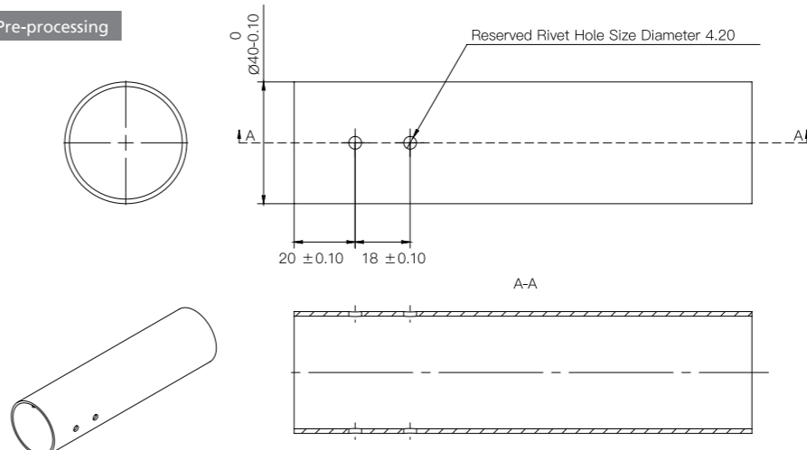
D40 Carbon Tube Pre-processing
